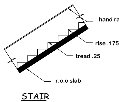
STAIR
