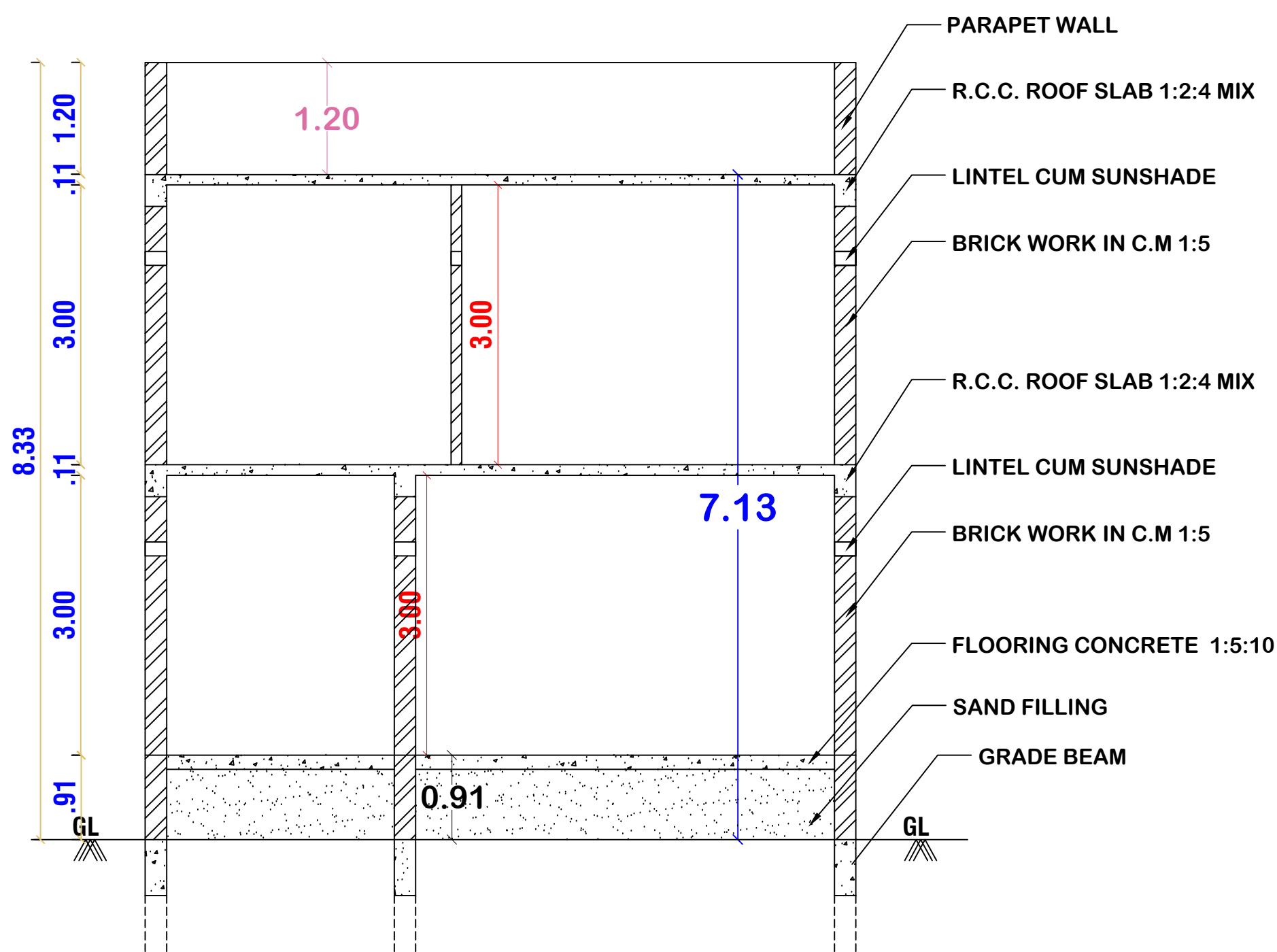
SECTION-AB
