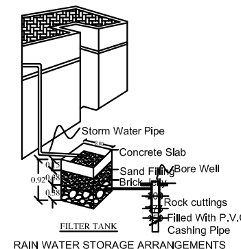
RAIN WATER STORAGE ARRANGEMENTS
