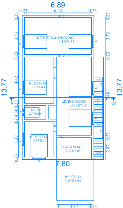
LOOR PLAN
