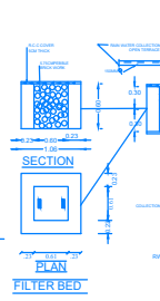
RAIN WATER HARVESTING PERCOLATION BED
