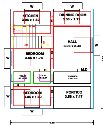
EXI. GROUND FLOOR PLAN
