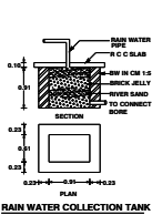
RAIN WATER COLLECTION TANK
