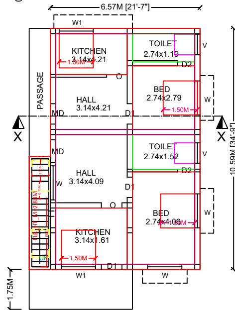
PROPOSED FF PLAN
