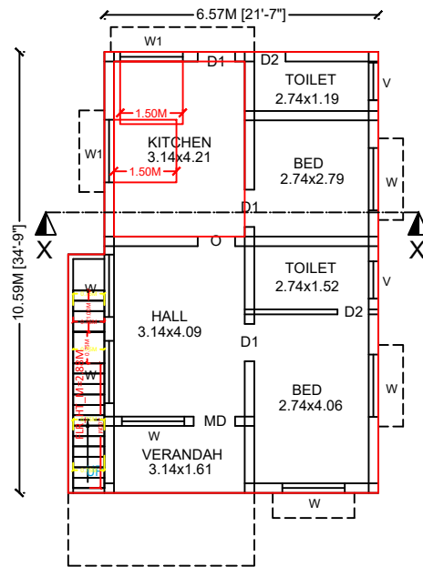
EXISTING GF PLAN
