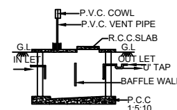
SEC. OF SEPTIC TANK SCALE (1:50)
