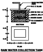
RAIN WATER COLLECTION TANK
