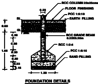
FOUNDATION DETAILS
