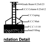
Foundation Detail
