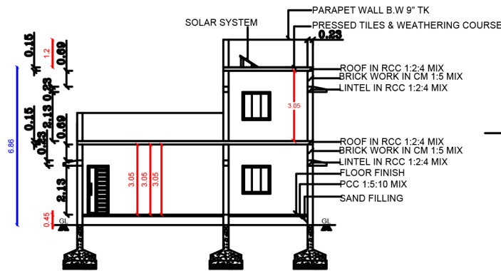
CROSS SECTION AB
