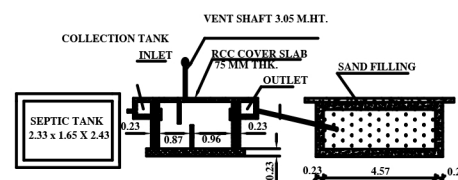
PLAN & SECTION ON SEPTIC TANK & DISP-TRENCH
