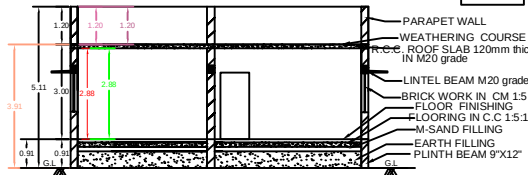
SECTION ON XX
