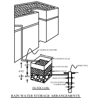
RAIN WATER STORAGE ARRANGEMENTS
