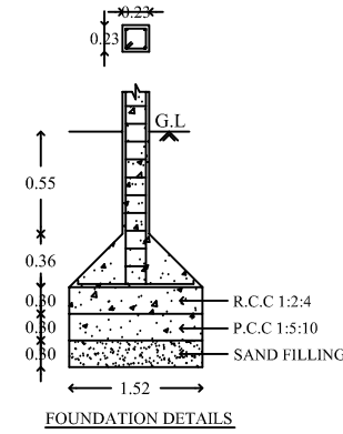
FOUNDATION DETAILS
