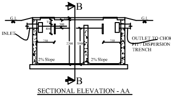
SECTIONAL ELEVATION-AA
