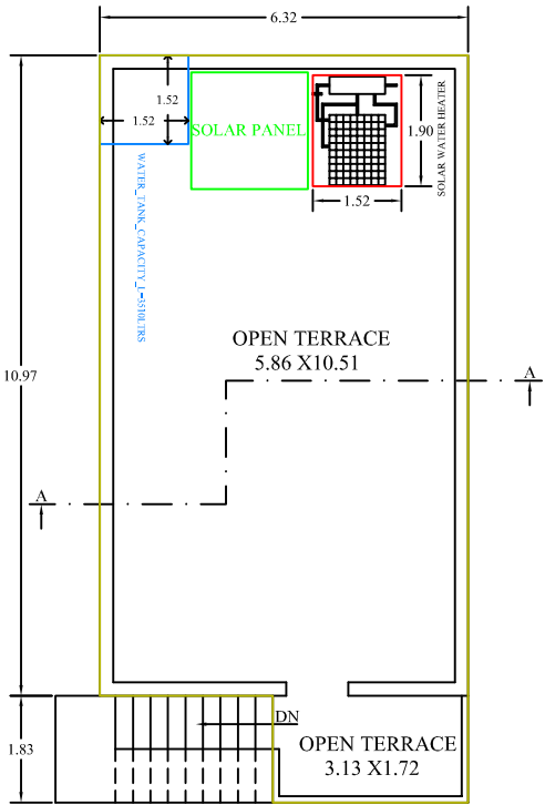
FLOOR TERRACE
