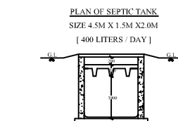
SECTIONAL ELEVATION-BB
