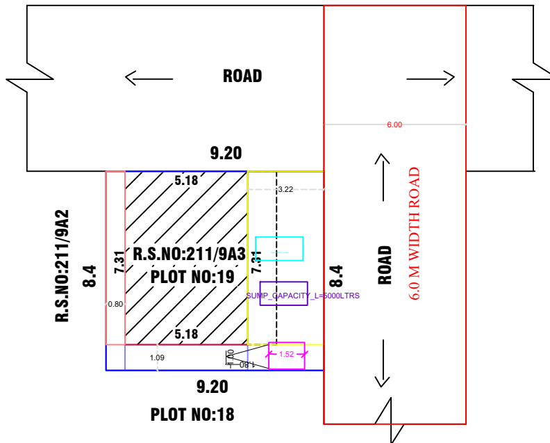
SITE PLAN
