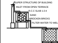
RAINWATER HARVESTING
