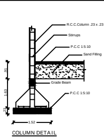
COLUMN DETAIL
