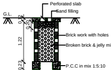
PERCOLATION PIT FOR 30 Sq. m.
