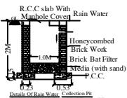
R.C.C. slab With Rain Water Collection (with sand) SCALE (1:50)
