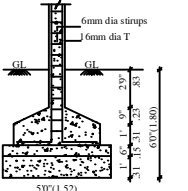
COLUMN FOUNDATION DETAIL SCALE (1:50)
