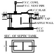
PLAN OF SEPTIC TANK SCALE (1:50)
