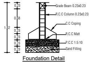
Foundation Detail
