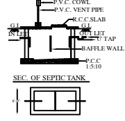
SEC. OF SEPTIC TANK SCALE (1:50)
