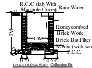
R.C.C. slab With Rain Water Collection SCALE (1:50)
