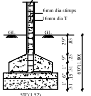
COLUMN FOUNDATION DETAIL SCALE (1:50)
