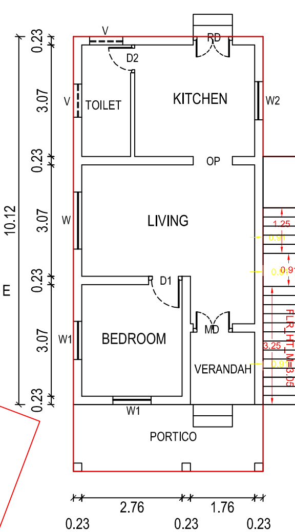
EXTG. GROUND FLOOR PLAN
