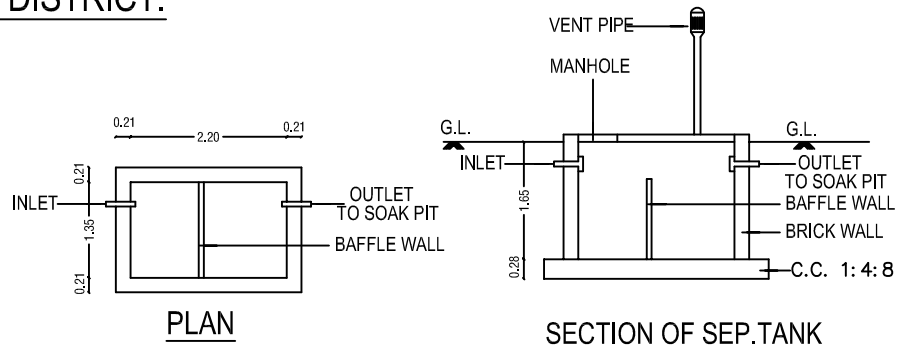
SEPTIC. TANK
