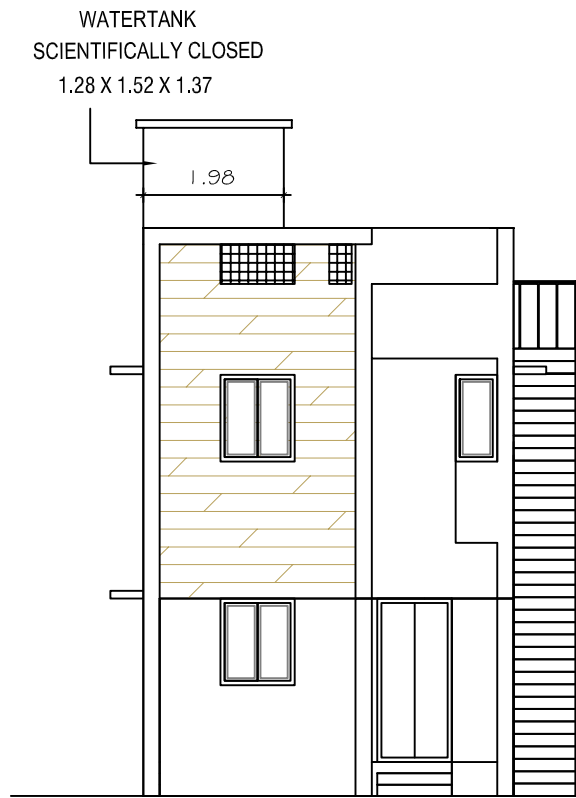
FRONT ELEVATION.
