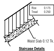
Staircase Details
