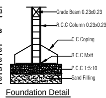
Foundation Detail
