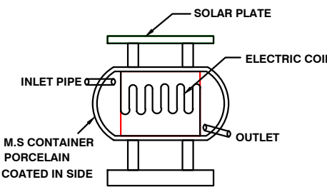
SOLAR SYSTEM
