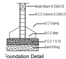
Foundation Detail
