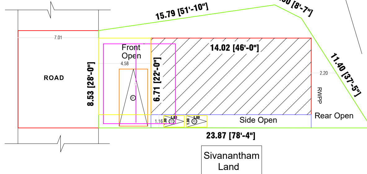
SITE PLAN
