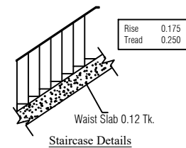
Staircase Details
