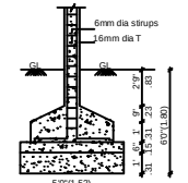
COLUMN FOUNDATION DETAIL SCALE (1:50)
