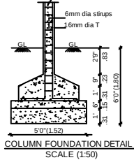
COLUMN FOUNDATION DETAIL SCALE (1:50)
