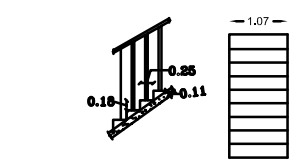
STAIRCASE DETAILS
