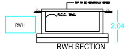
RWH SECTION
