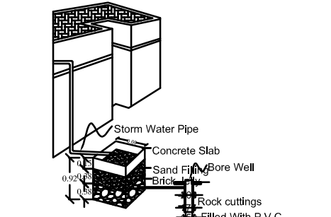
RAIN WATER STORAGE ARRANGEMENTS
