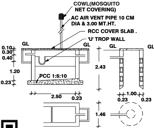
CROSS SECTION OF ST&SP.
