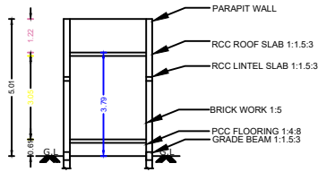
SECTION ON XX
