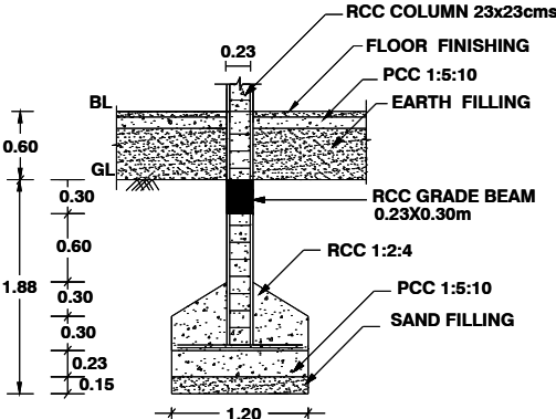
FOUNDATION DETAILS
