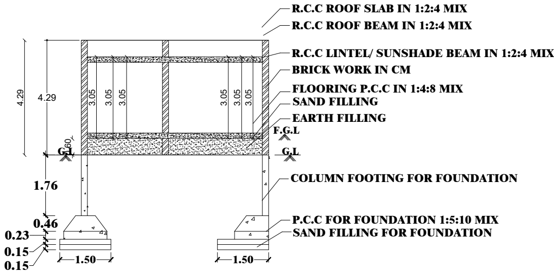
SECTION ON-AA
