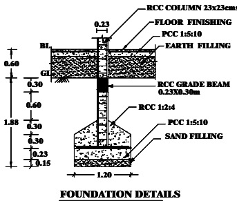
FOUNDATION DETAILS
