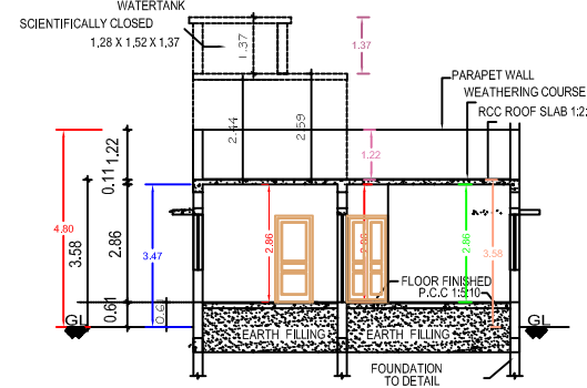
SECTION "A-B"
