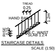
STAIRCASE DETAILS SCALE (1:50)
