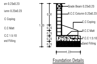
Foundation Details
