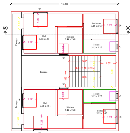
PRO. FIRST FLOOR PLAN
