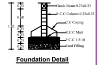
Foundation Detail
