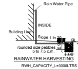
RAINWATER HARVESTING RWHL_CAPACITY_L=3000L,TRS
