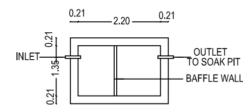
PLAN SEPTIC. TANK
