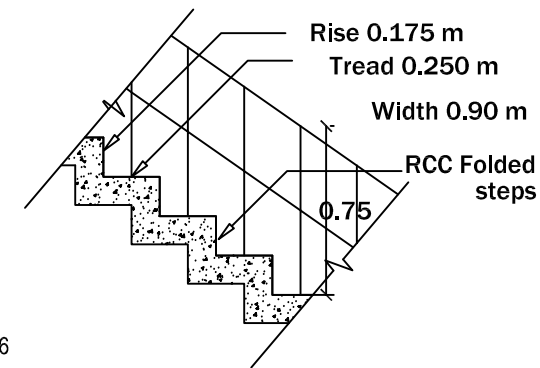
STAIRCASE DETAILS
