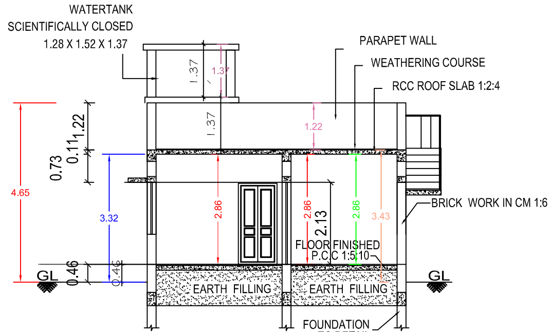
SECTION "A-B"
