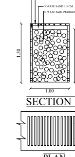
RAIN WATER HARVESTING PERCOLATION BED
