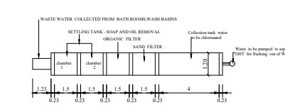
10.09 PLAN WASTE WATER RECYCLING SYSTEM
