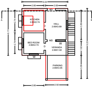
EXI.GROUND FLOOR PLAN BLOCK-1
