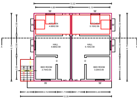
EXI.GROUND FLOOR PLAN BLOCK-2
