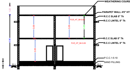
SECTION FOR BLOCK-2
