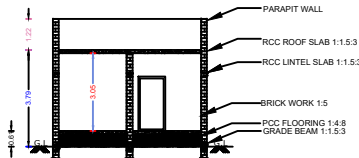
SECTION FOR BLOCK-1
