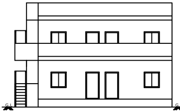
ELEVATION FOR BLOCK-2
