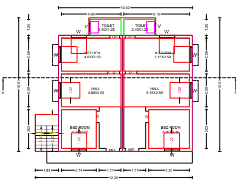
PRO.FIRST FLOOR PLAN BLOCK-2
