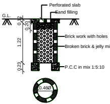
PERCOLATION PIT FOR 30 Sq. m. (Scale:- 1:50)
