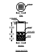
RAINWATER HARVESTING
