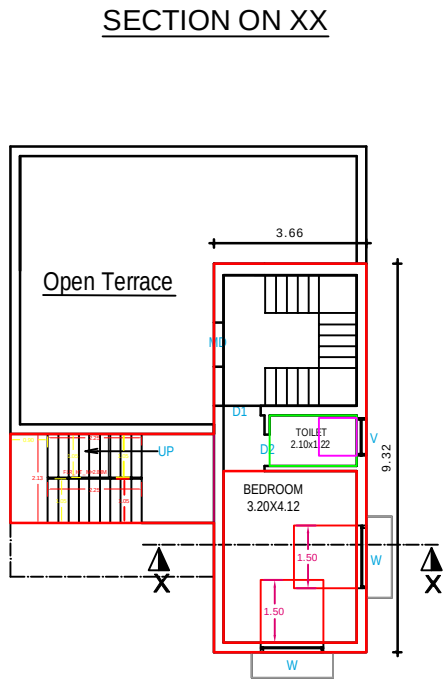
PRO. FIRST FLOOR PLAN
