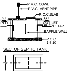
PLAN OF SEPTIC TANK SCALE (1:50)
