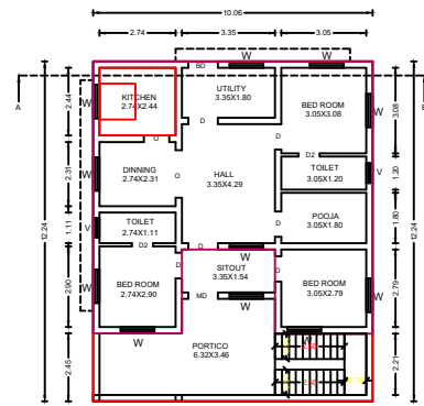
EXI.GROUND FLOOR PLAN
