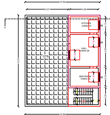
PRO.SECOND FLOOR PLAN
