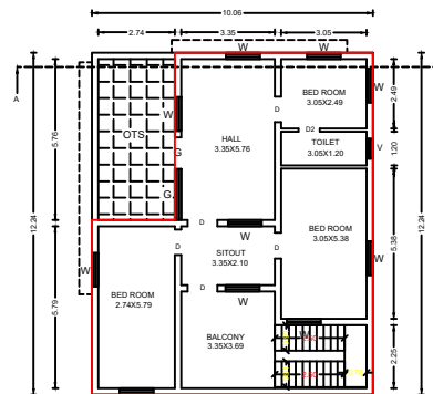
EXI.FIRST FLOOR PLAN
