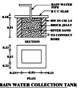
RAIN WATER COLLECTION TANK
