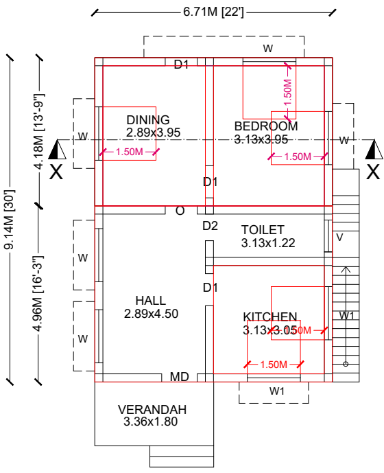
EXISTING & PROPOSED GF PLAN
