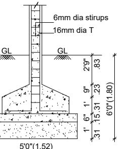
COLUMN FOUNDATION DETAIL SCALE (1:50)
