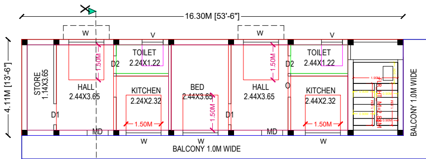
PROPOSED FIRST FLOOR PLAN
