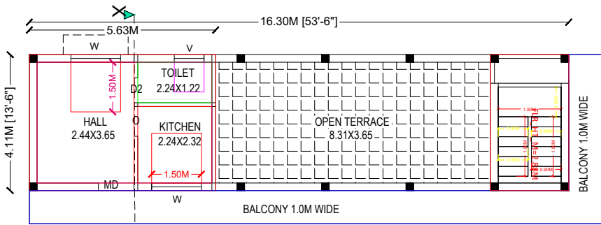
PROPOSED SECOND FLOOR PLAN
