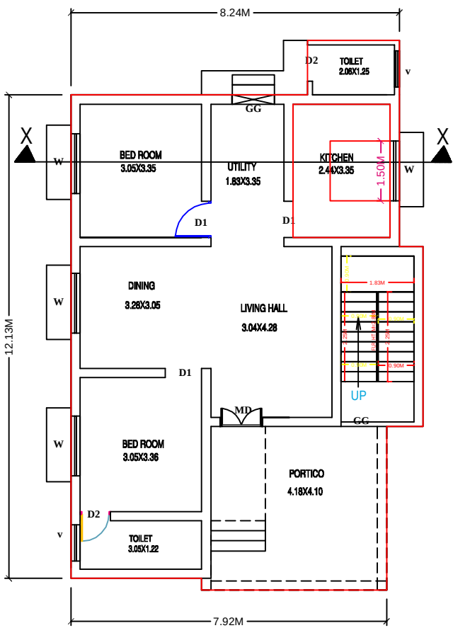
EXT. GROUND FLOOR PLAN
