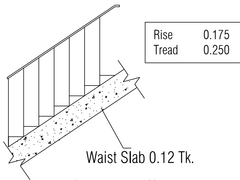
Staircase Details
