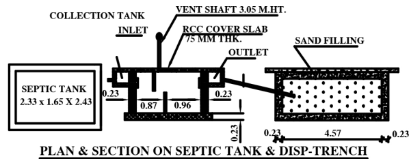
PLAN & SECTION ON SEPTIC TANK & DISP-TRENCH
