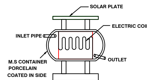
SOLAR SYSTEM
