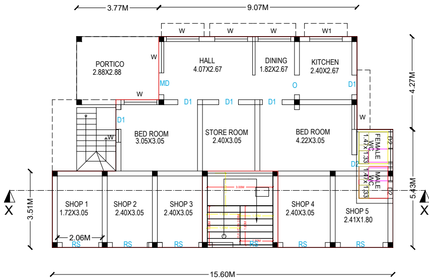
EXISTING. GF PLAN
