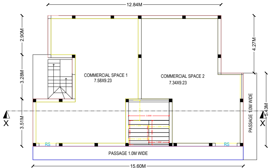
PROPOSED FF PLAN
