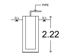
DETAILS OF RAINWATER COLLECTION TANK
