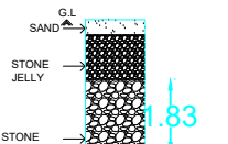
RAINWATER HARVESTING PIT [ RWHP ]
