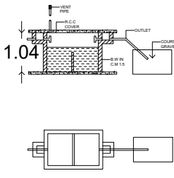
SEPTIC TANK & D-TRENCH DETAILS [ NOT TO SCALE ]
