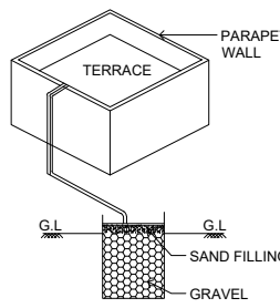
COLLECTION SUMP FOR HARVESTING FOR TERRACE
