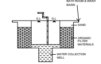
PLAN AND SECTION OF ORGANIC FILTRATIONS SUMP WITH COLLECTION WELL
