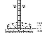
COLUMN DETAILS [ NOT TO SCALE ]
