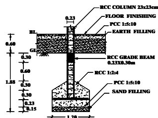
FOUNDATION DETAILS
