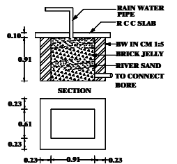
RAIN WATER COLLECTION TANK
