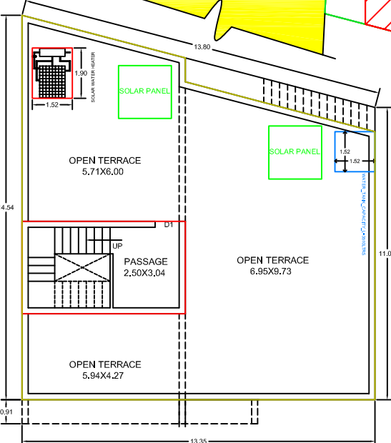
TERRACE FLOOR
