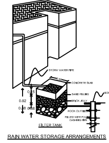
RAIN WATER STORAGE ARRANGEMENTS
