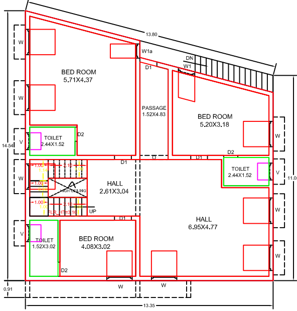
PRO-FIRST FLOOR
